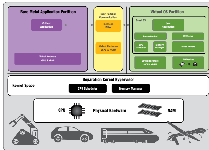
Figure 1: Platform integrity through isolated domains
