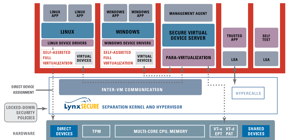
Figure 3: LynxSecure architecture
