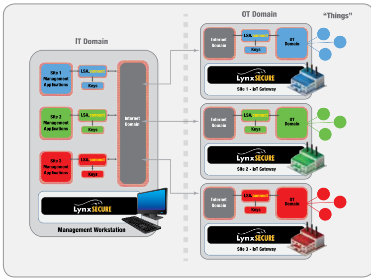
Figure 2: Networking integrity using multi-channel secure communications
